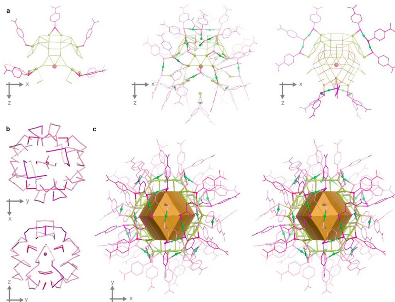
Figure 3. Configuration of ligands (p-MBA) on \text{Au}_{146}(\text{p-MBA})_{57} . (a) Distribution of the three types of staples on the core surface of \text{Au}_{146}(\text{p-MBA})_{57} . Bridging motifs (left) in pink, monomeric staples (center) in light pink, and dimeric staples (right) in purple. (b) Rotational symmetric distribution of staples. Screw axis parallel to z -axis bisecting the twin plane ( xz -plane). (c) Stereoscopic view of \text{Au}_{146}(\text{p-MBA})_{57} displaying all different types of staples; J27-2 atoms are displayed as solid surface.
