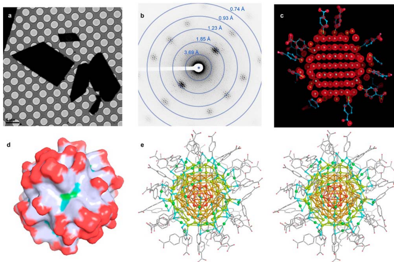
Figure 1. MicroED and X-ray determination of the crystal structure of \text{Au}_{146}(\text{p-MBA})_{57} . (a) Transmission electron micrograph of \text{Au}_{146}(\text{p-MBA})_{57} crystals and (b) typical MicroED data extending well beyond 1 Å. (c) MicroED density map (2Fo-Fc, contoured at 2\sigma ), shown as red mesh, identifies atomic positions of Au (white spheres) and S (yellow spheres) atoms. Ligands (p-MBA) are shown as blue framework. (d) Surface representation of the cluster with oxygen in red, carbon in white, sulfur in cyan, and gold in green. The full set of p-MBA ligands was determined using X-ray data. (e) Stereoscopic representation of the cluster including all gold atoms and p-MBA ligands. Gold atoms colored by shells for visualization purposes (see Figure 2).
